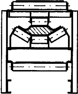
TYPICAL INCLINED SECTION
