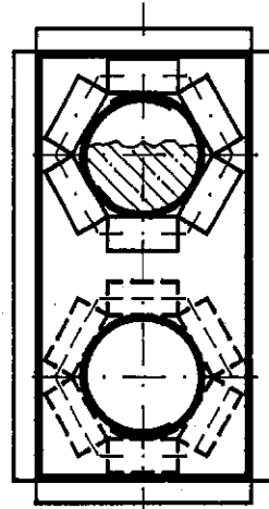
TYPICAL CROSS SECTION
